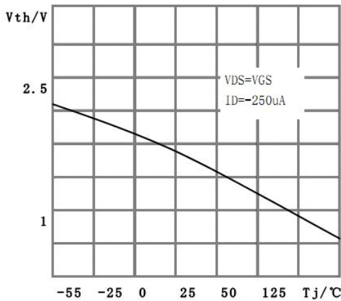
Figure 3. Gate Threshold Variation with Temperatures
