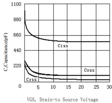
Figure 4: Capacitance vs. Gate-Source Voltage
